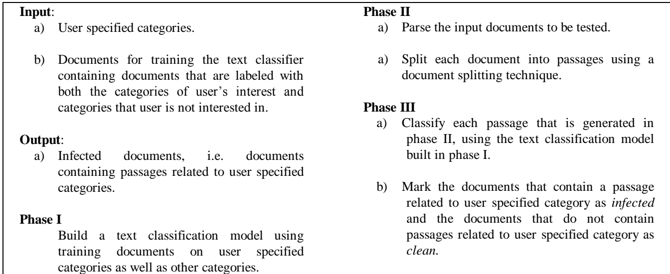
Figure 1. Pseudocode of the three phase methodology for passage detection
