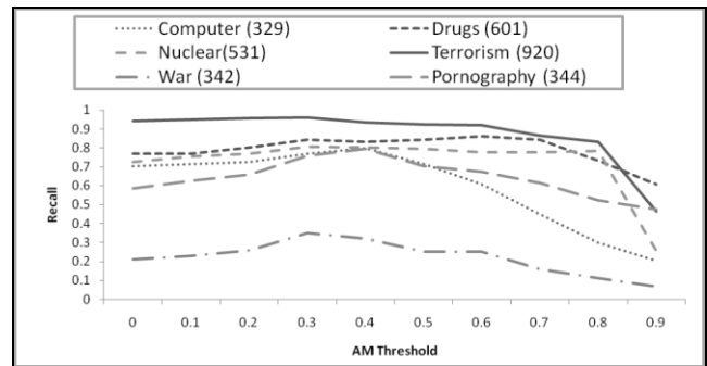
Figure 13. Effects of category distribution in training documents on KDP recall using 20 Newsgroups dataset
