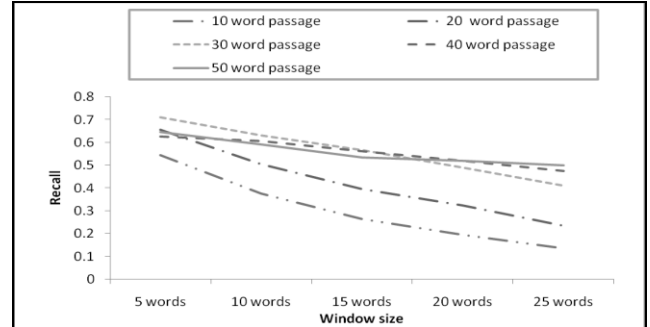
Figure 11. Recall values with respect to various passage lengths for different window sizes on OWP approach using 20 Newsgroups dataset
