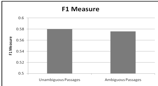
Figure 14. Effects of ambiguous passages on S-PCP in KDP approach using 20 Newsgroups
