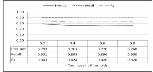
Figure 10. Effects of term weight thresholds on KDP approach using 20 Newsgroups dataset for PD task
